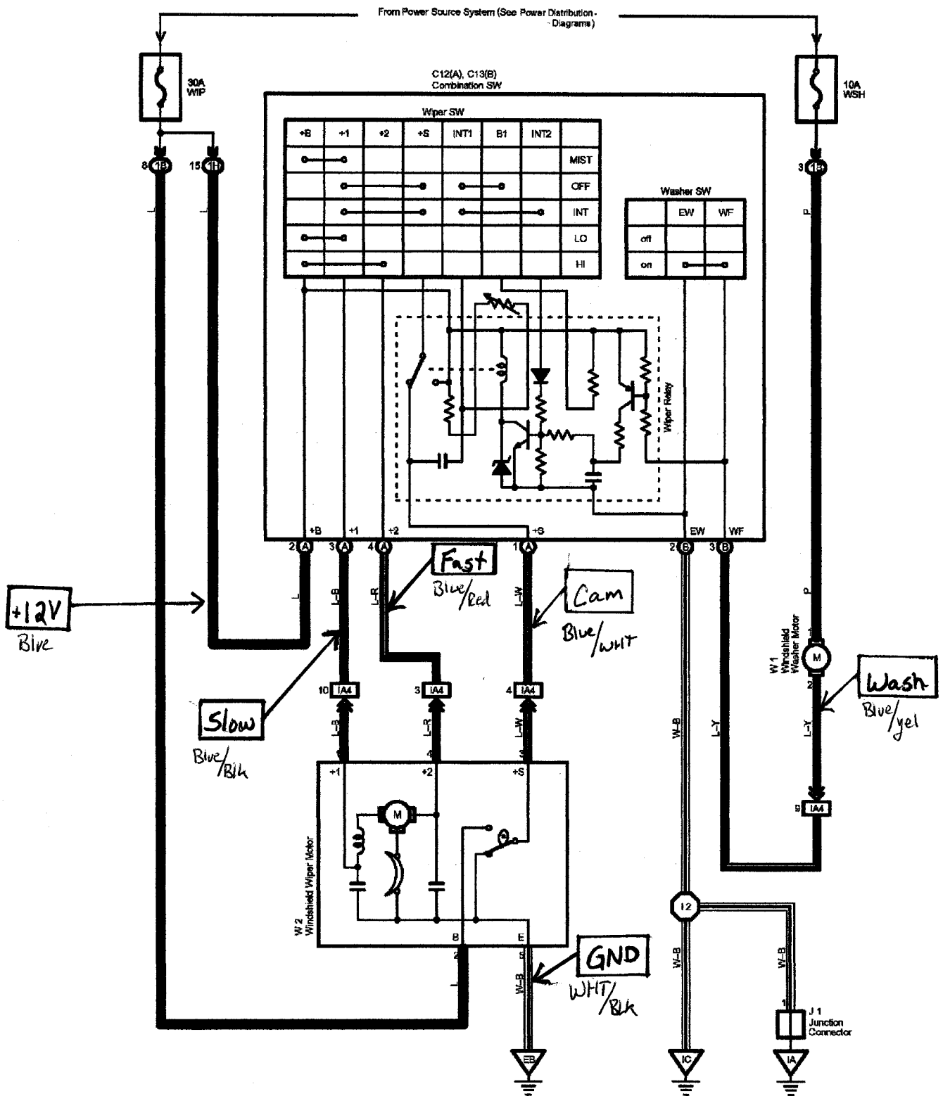
Wiper And Washer With INT Time SW
