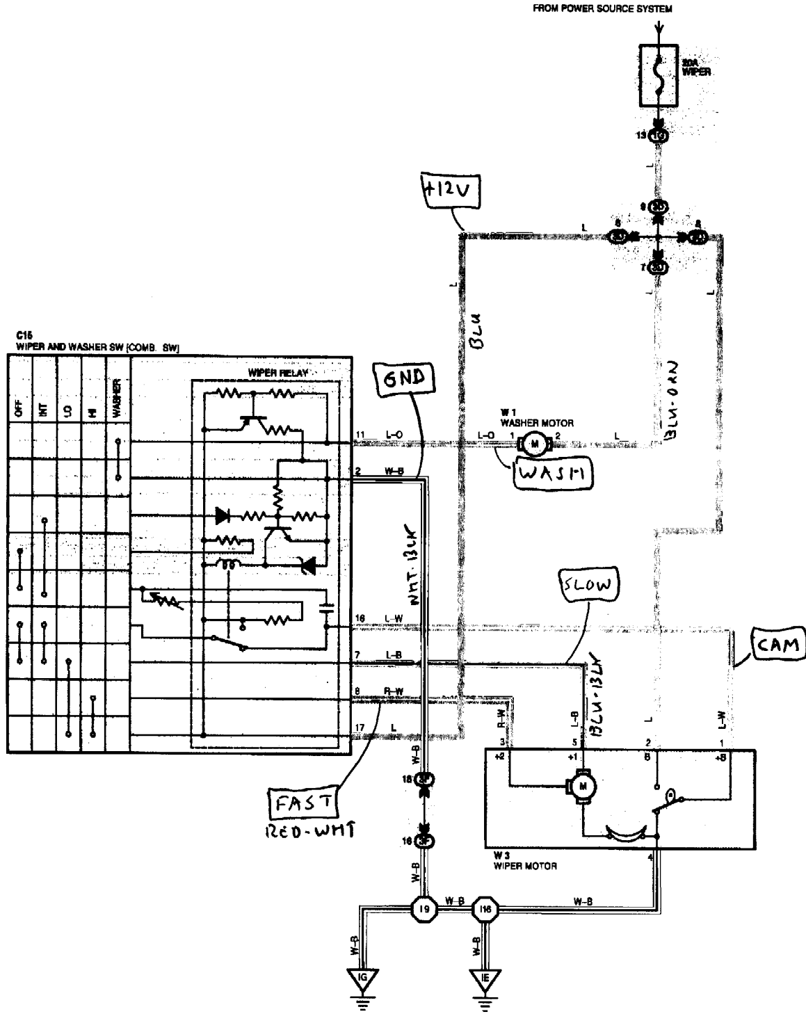
Wiper And Washer (w/ INT Time SW Mechanism)
