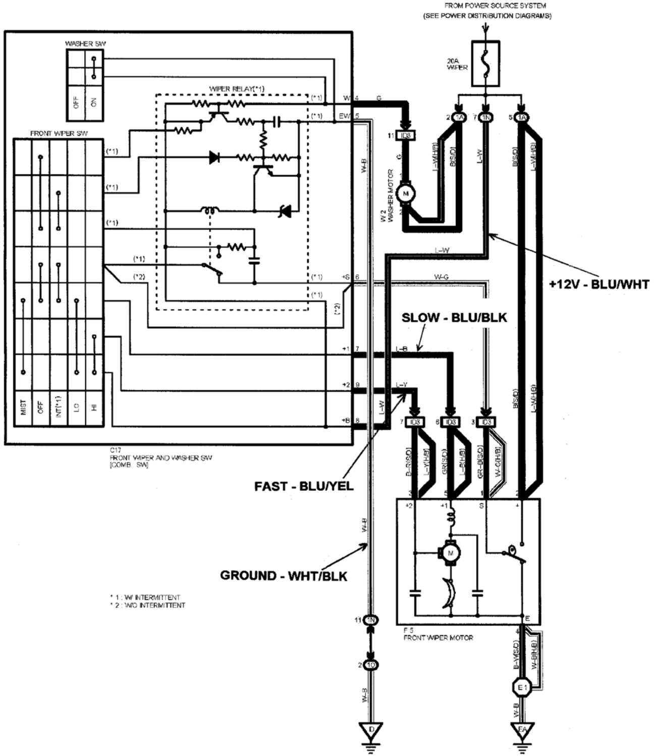
Front Wiper And Washer
