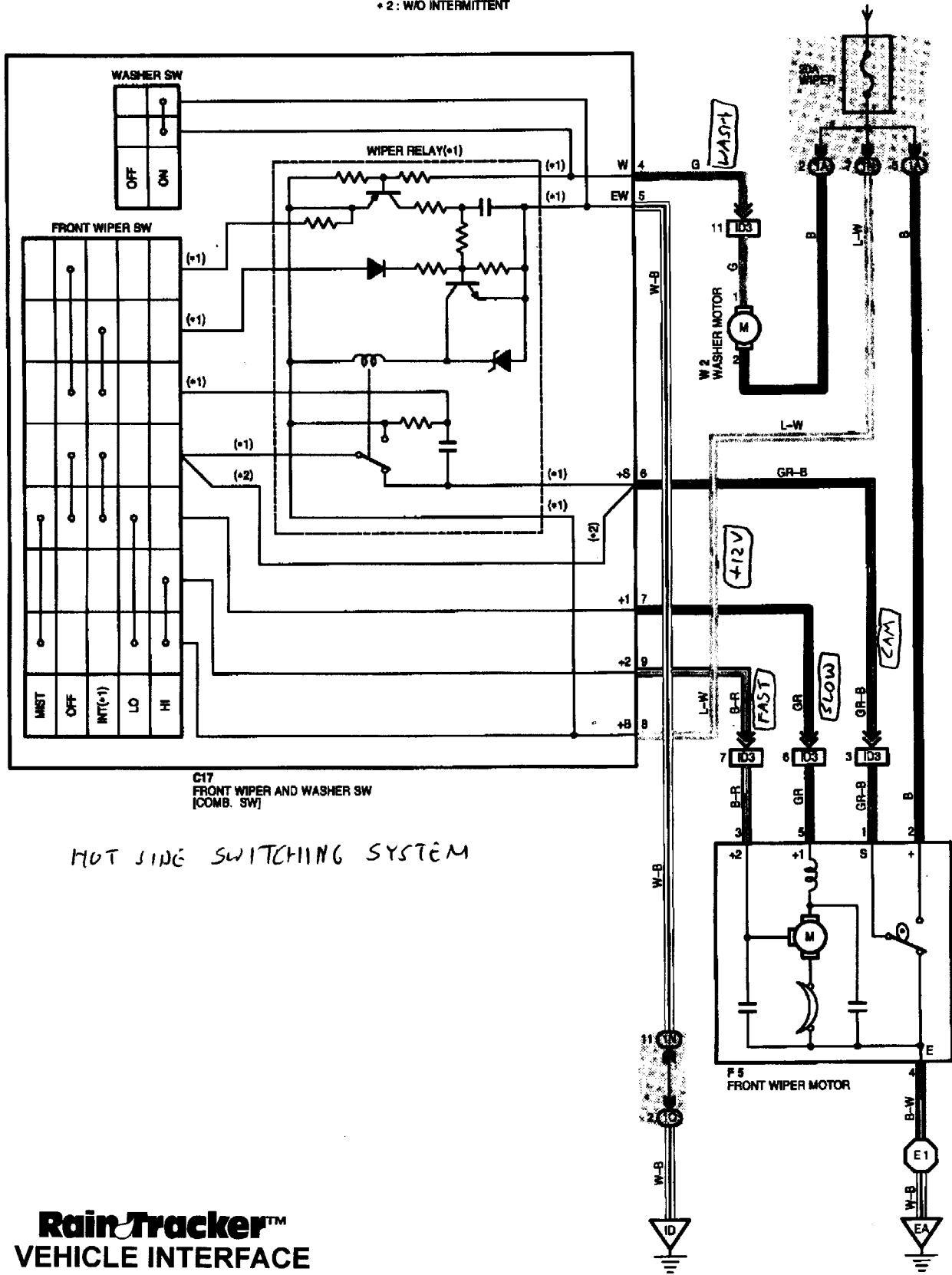
Front Wiper And Washer
