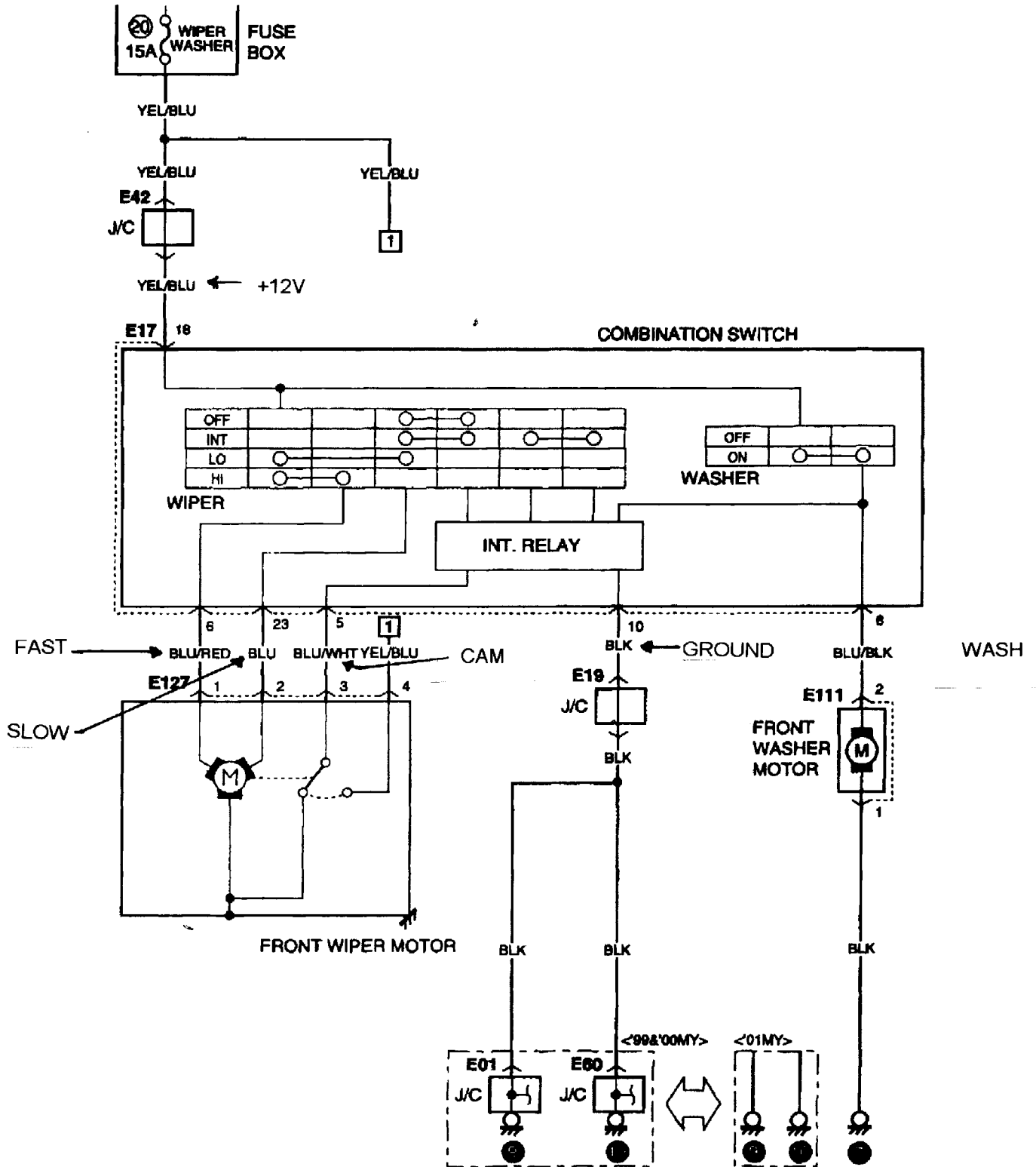
B-3 Windshield Wiper And Washer
