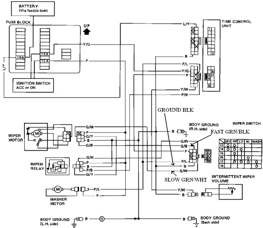
Windshield Wiper/Washer System, Front
