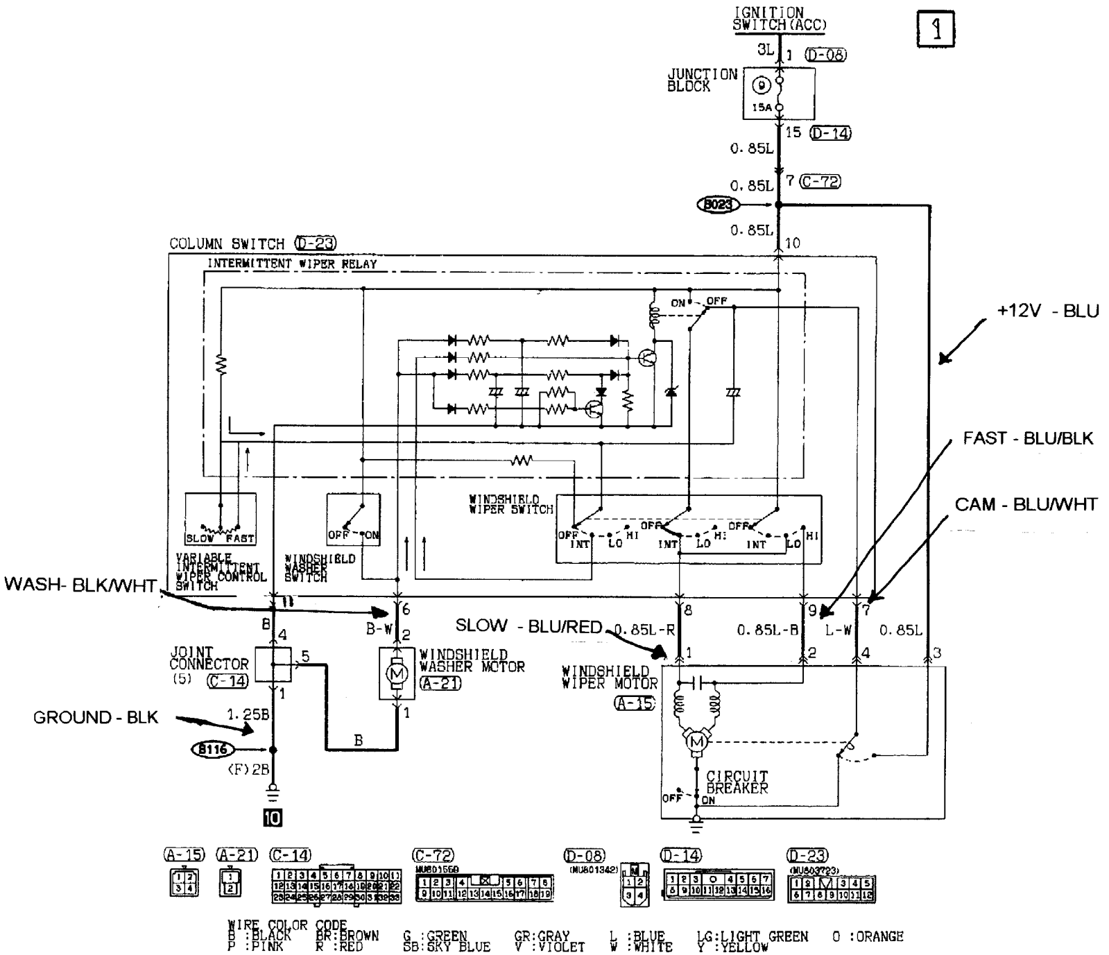
Windshield Wiper And Washer
