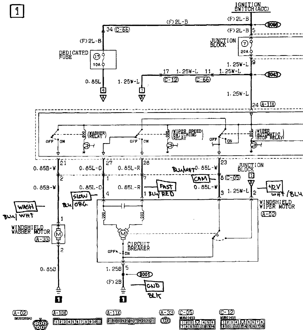
Windshield Wiper And Washer Part 1
