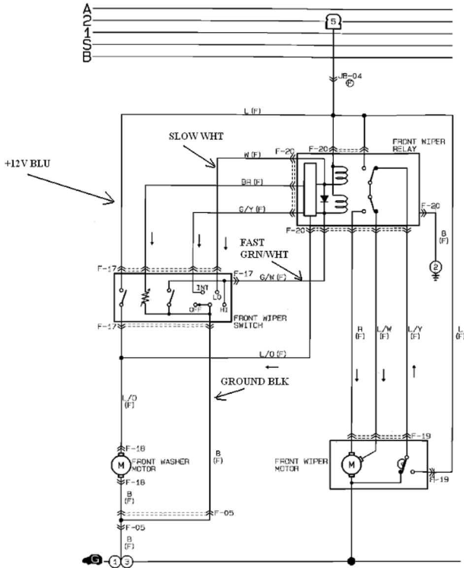
Windshield Wiper/washer
