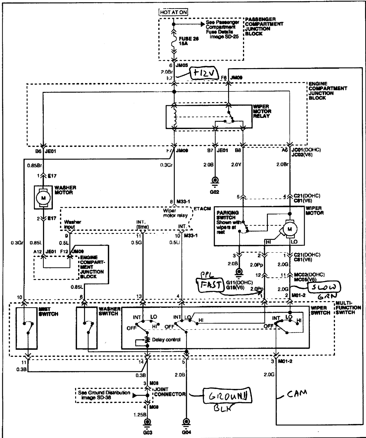
Image SD-132 - ETACS (Electronic Time & Alarm Control System) (1)
