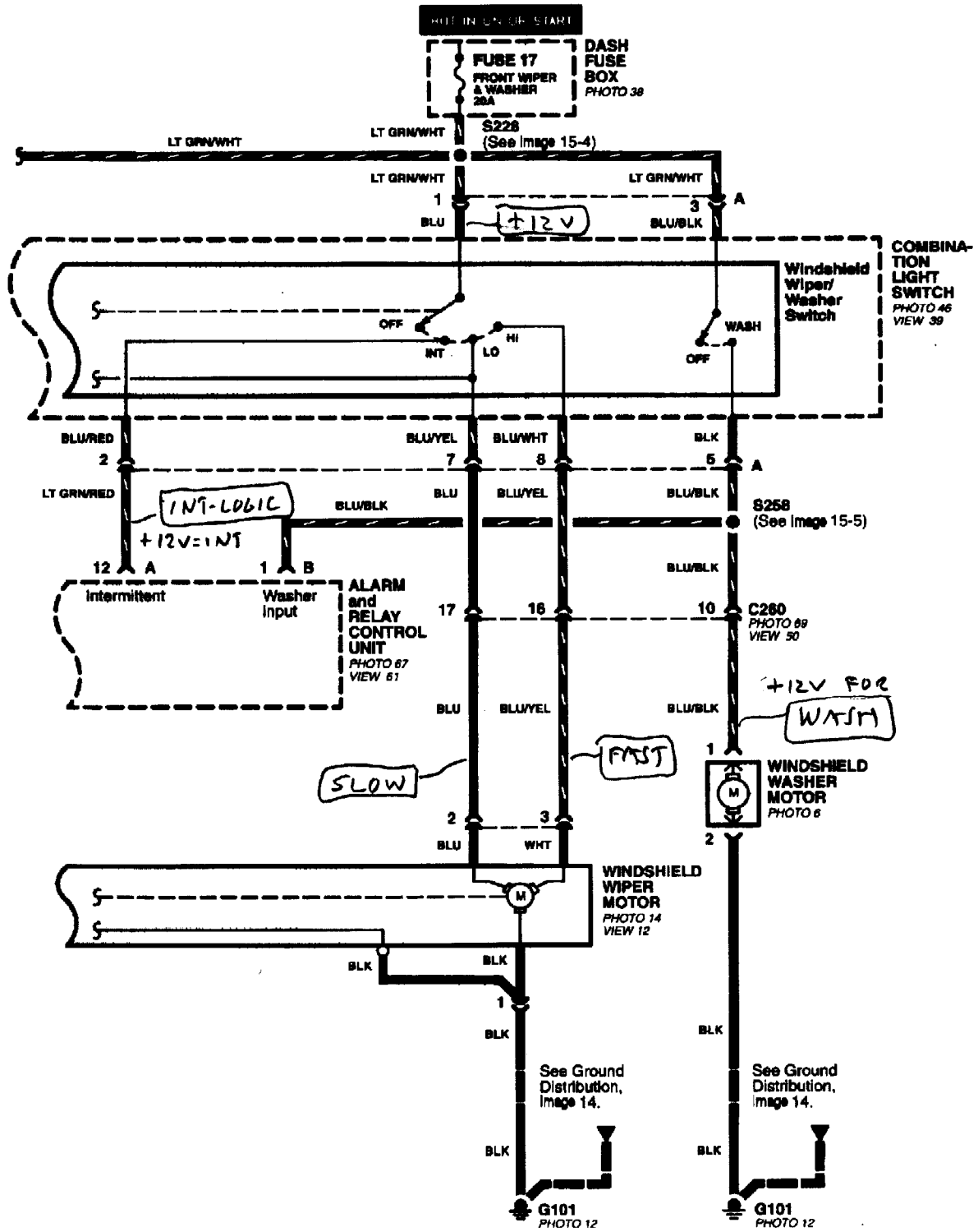
Front Wiper/Washer Image 91-1
