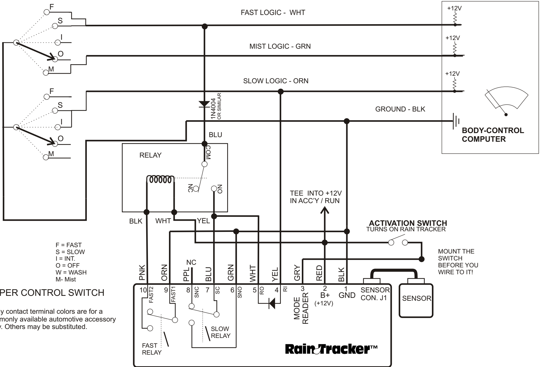
RAIN TRACKER INTERFACE WIRING DIAGRAM WIPER SYSTEM CLASS: Honda Logic Diagram
