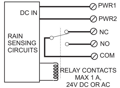
EQUIVALENT SCHEMATIC
