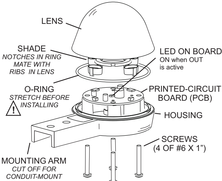
EXPLODED VIEW
